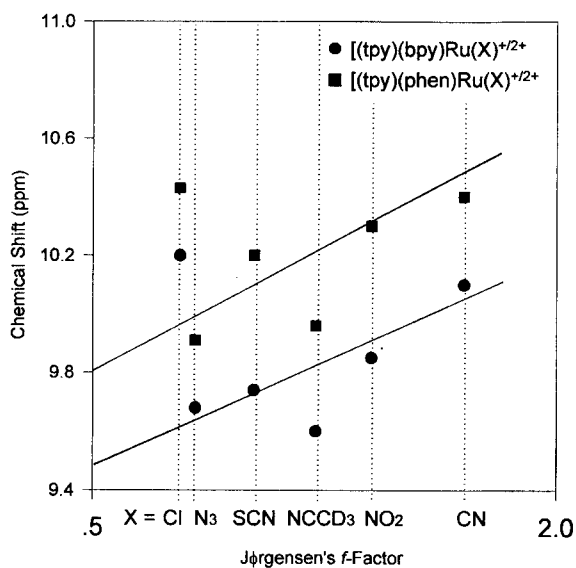
Figure 1. The ligand field strength vs the chemical shift to the particular proton of each ligand bpy and phen in [(\text{tpy})(\text{bpy})\text{Ru}(\text{X})]^{+2+} and [(\text{tpy})(\text{phen})\text{Ru}(\text{X})]^{+2+} ( \text{X}=\text{Cl} , \text{CN} , \text{N}_3 , \text{NCCD}_3 , \text{NO}_2 , \text{SCN} ) complexes in \text{CD}_3\text{CN} ; \bullet=[(\text{tpy})(\text{bpy})\text{Ru}(\text{X})]^{+2+} , \blacksquare=[(\text{tpy})(\text{phen})\text{Ru}(\text{X})]^{+2+} .
