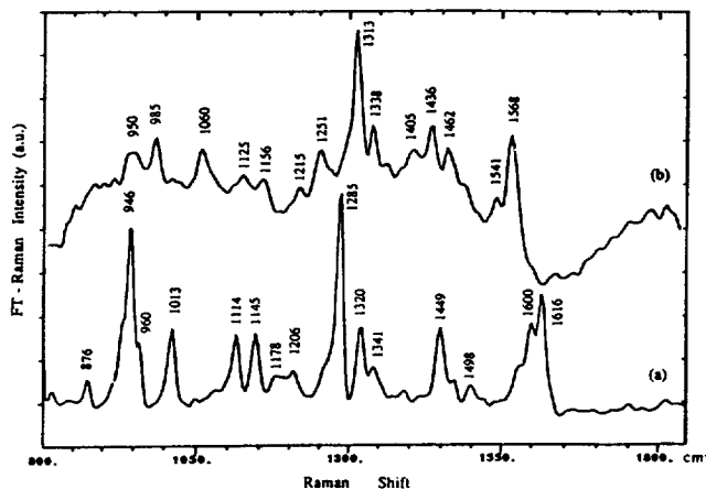
Figure 1. FT-Raman spectra of cationic state (a) and sodium salt (b) of dopamine in powder state in ordinary melting capillary tube. Nd:YAG laser 1064 nm excitation, 0.1 watt power at sample, spectral resolution 10 \text{cm}^{-1} , 1000 times coadded.
