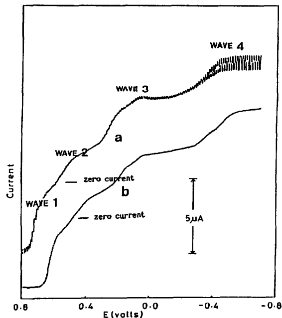
Figure 1. Conventional (a) and rapid (drop time: 1.06 sec) (b) polarograms of \text{SpCuCl}_2 (solvent; acetone/0.1 M TEAP, reference electrode; Ag/AgCl in 1 M LiCl).
