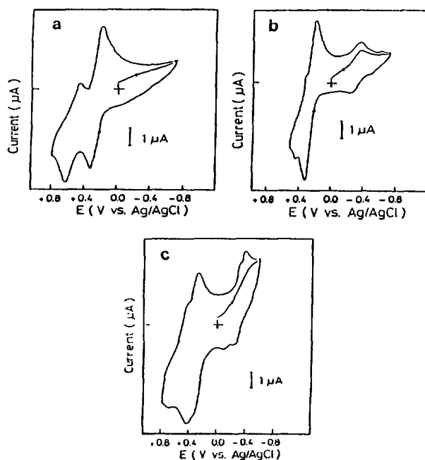
Figure 8. Cyclic voltammogram of 1 \times 10^{-3} \text{M} \text{SpCuBr}_2 with platinum electrode (a), HMDE (b), and Pt electrode in the cell containing Hg pool (c) (solvent; DMF/0.1 M TEAP, scan rate; 100 mV/sec).
