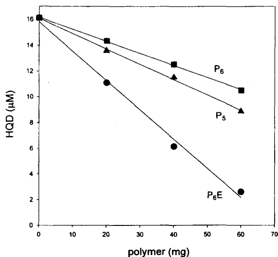
Figure 1. Results of equilibrium binding experiments with HQD: The concentration of HQD in solution as a function of added polymer: P 5 (nonimprinted polymer), P 6 (HQD-imprinted and unextracted polymer), P 6E (HQD-imprinted and extracted polymer).
