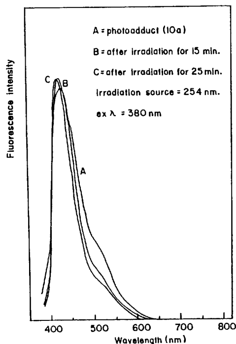
Figure 3. Photodecomposition of thioxanthone-cyclohexene photoadduct (10a) in dichloromethane.
