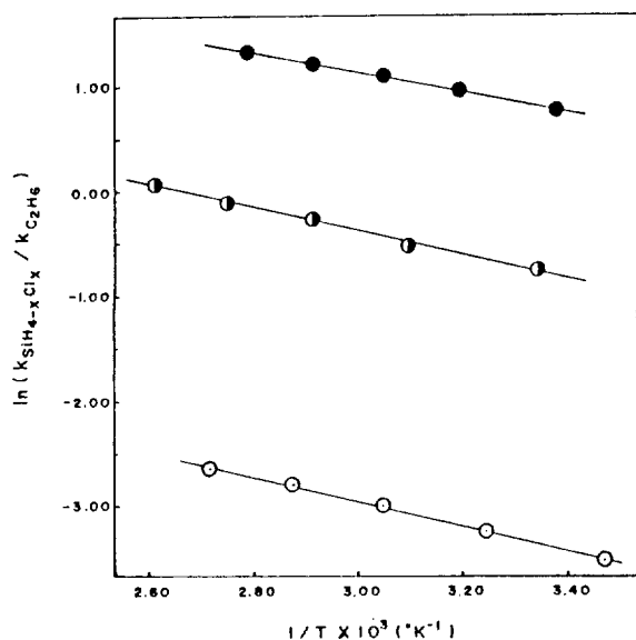
Figure 1. The photochlorination rate constant ratios between chlorosilanes and ethane as a function of reaction temperature at 337.1 nm: (○) \text{SiH}_4 ; (◐) \text{SiHCl}_3 ; (●) \text{SiH}_2\text{Cl}_2 .
