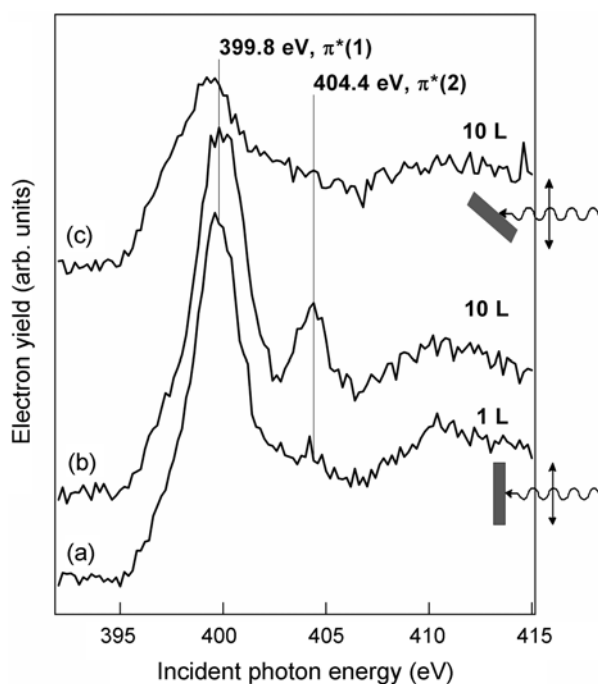
Figure 3. Nitrogen K-edge NEXAFS features of NO x species adsorbed on a VO/V(110) surface. Spectra (a) and (b) were recorded with the incident photon beam normal to the surface. Spectrum (c) was recorded with the incident photon beam glancing to the surface by 20°.
