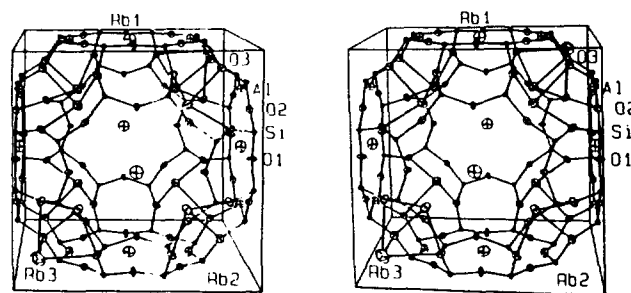
Figure 2. A stereoview of a large cavity in \text{Rb}_{13.5}\text{-A} . Eight Rb species at Rb(2), two Rb species at Rb(3), and three \text{Rb}^+ ions at Rb(1) are shown. Ellipsoids of 20% probability are used.
