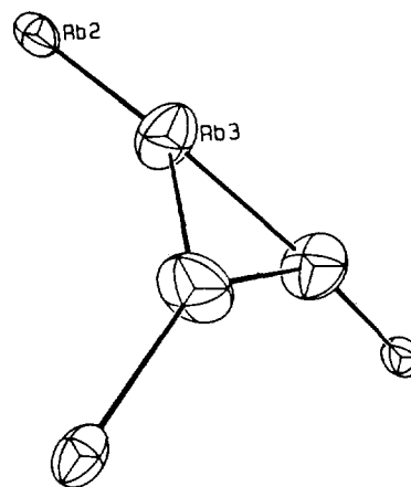
Figure 6. The trigonal rubidium cluster, (\text{Rb}_6)^{4+} , in \text{Rb}_{14}\text{-A} . The \text{Rb}(3) 's are in the sodalite unit and the \text{Rb}(2) 's are in the large cavity. Ellipsoids of 20% probability are used.
