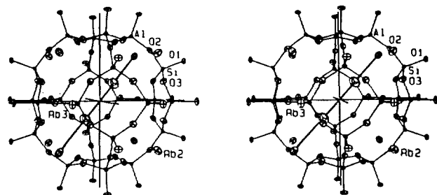
Figure 3. A stereoview of a sodalite cavity in \text{Rb}_{13.5}\text{-A} . A linear (\text{Rb}_4)^{3+} cluster is shown. Ellipsoids of 20% probability are used.
