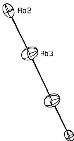
Figure 4. The linear rubidium cluster, (\text{Rb}_4)^{3+} . Ellipsoids of 20% probability are used.
