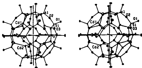
Figure 1. A stereoview of the sodalite unit of fully dehydrated \text{Cd}_6\text{-A} . Two \text{Cd}^{2+} ions at Cd(1) and four \text{Cd}^{2+} ions at Cd(2) are shown. Ellipsoids of 20% probability are used.
