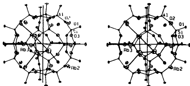
Figure 5. A stereoview of a sodalite cavity in \text{Rb}_{14}\text{-A} . A trigonal (\text{Rb}_6)^{4+} cluster is shown. Ellipsoids of 20% probability are used.
