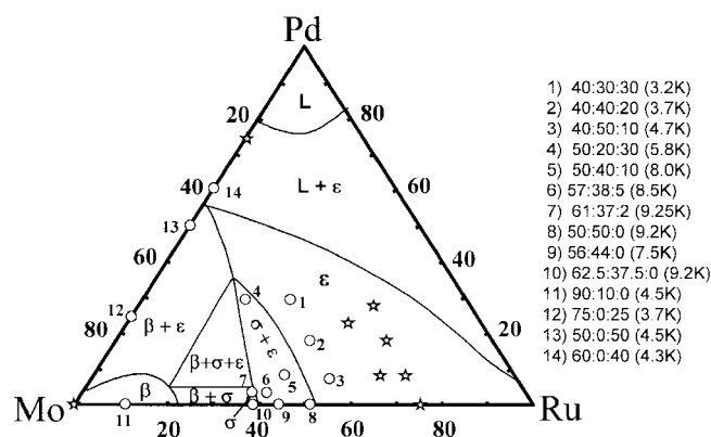
Figure 4. Superconducting composition in the phase diagram of ternary and binary alloy (Mo-Ru-Pd), 1700 °C. The asterisk marks denote the absence of superconductivity above 2 K.
