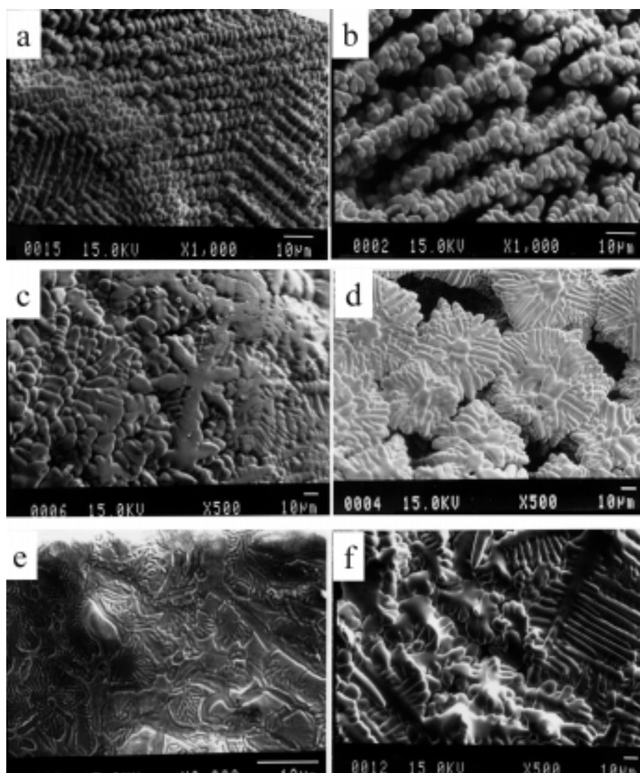
Figure 2. SEM images of the top surface of ternary and binary alloys in Mo-Ru-Pd. a and b are e-phases, c and d are a mixture of the \epsilon - and \sigma -phases, e is the \sigma -phase and f is the \beta -phase. (a. 40:40:20; b. 40:30:30; c. 50:20:30; d. 50:40:10; e. 62.5:37.5:0; f. 90:10:0)
