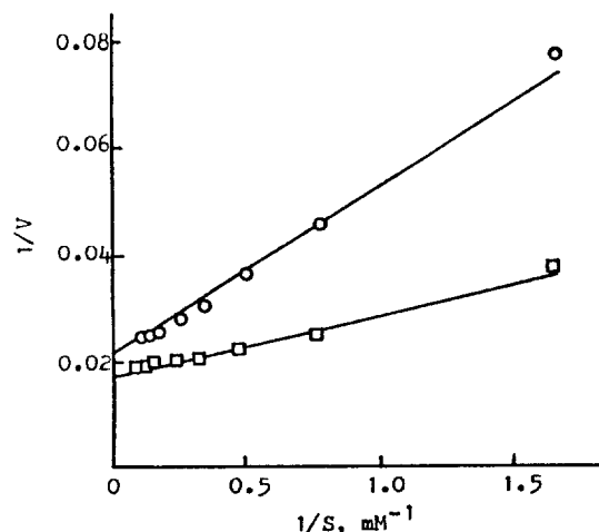
Figure 7. Lineweaver-Burk plot of the substrate dependence of phospholipase D activity. PC-PA liposome system (○-○); PC-SDS mixed micelle system (□-□).
