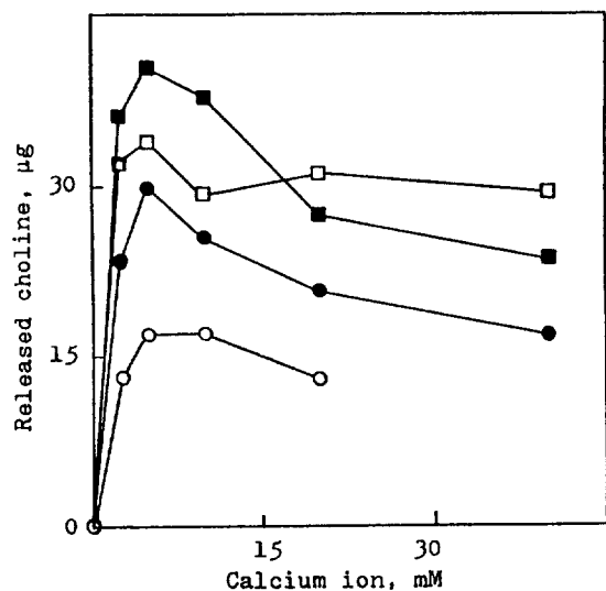
Figure 5. The effect of Ca ion concentration on the activity of phospholipase D. phosphatidylcholine 1 mM (2.5 \mu mole) (○-○); 2 mM (5 \mu mole) (●-●); 4 mM (10 \mu mole) (□-□); 8 mM (20 \mu mole) (■-■).
