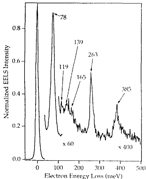
Figure 3. Vibrational EEL spectra for \text{CH}_2\text{CO} (2 L exposure) on Ag(111) at 87 K.
