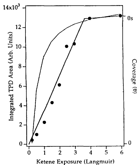
Figure 2. Integrated TPD area of the mass 42 peak as a function of ketene exposures. The curved line represents the fit to Langmuir kinetics model. The straight line for 0 \leq L_{\text{exp}} \leq 3.66 L is \theta = 0.274 L_{\text{exp}} \theta_s , where \theta_s is the saturation coverage defined by the coverage at 6 L exposure.
