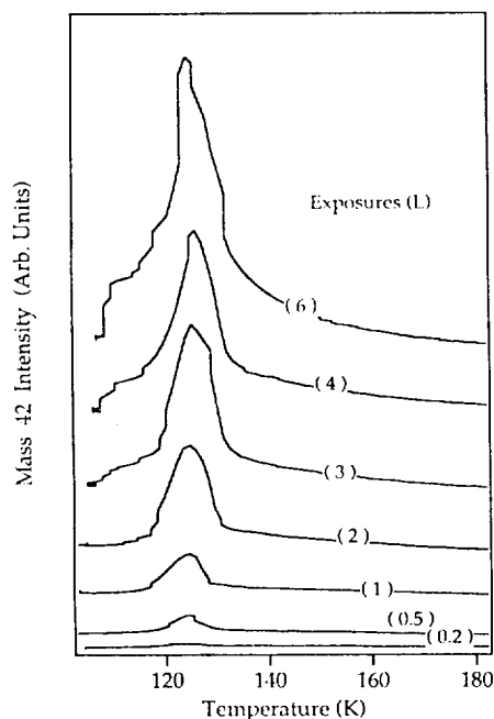
Figure 1. Temperature programmed desorption spectra (mass 42, 1 Ks -1 ) for 0.2 L~6 L CH 3 CO exposure on Ag(111).
