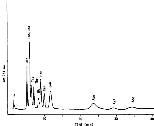
Figure 5. Isocratic elution profiles of a mixture of nucleosides and bases on a PVA column. Column, 9 \mu m Asahipak GS 320H; mobile phase, 10 mM SDS (pH 3.4). Other Chromatographic conditions are the same as in Figure 1.
