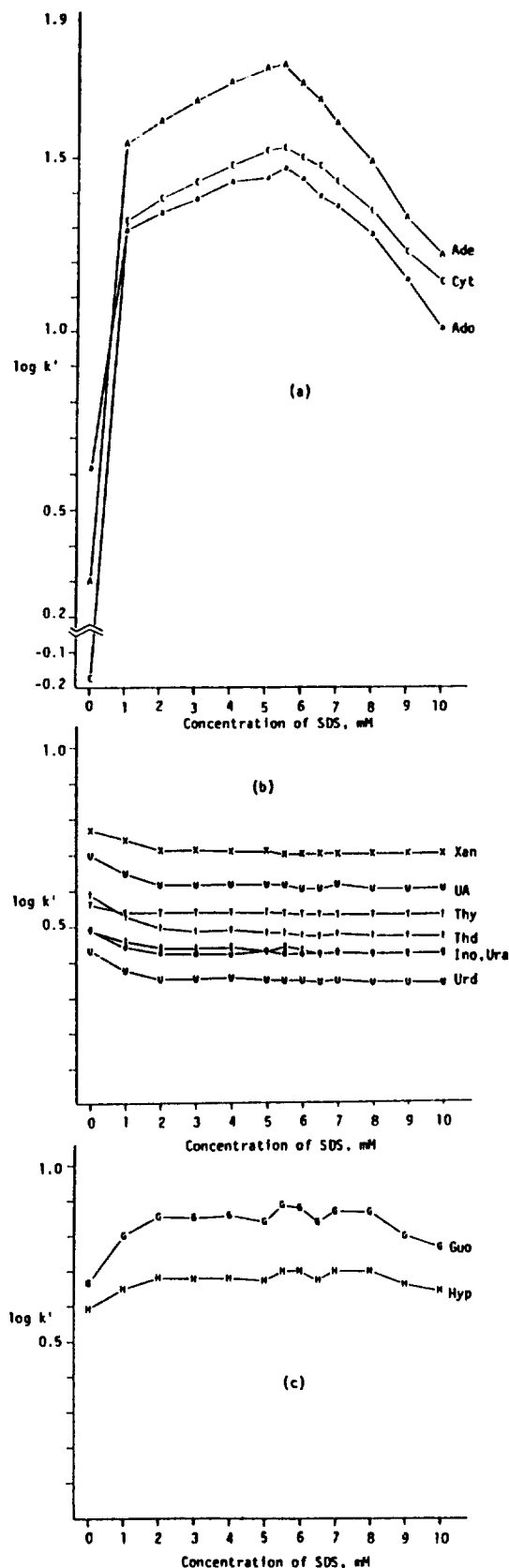
Figure 4. Effect of SDS concentration on the capacity factors of (a) Ado, Cyt and Ade, (b) Xan, UA, Thy, Thd, Ino, Ura and Urd, (c) Hyp and Guo. Mobile phase, aqueous SDS solutions (pH 3.4). Other chromatographic conditions are the same as in Figure 1.
