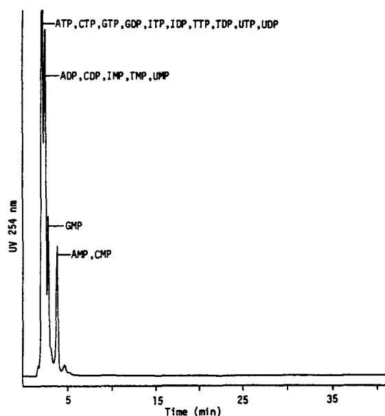
Figure 2. Isocratic elution profiles of a mixture of nucleotides. Mobile phase, 10 mM SDS (pH 3.4). Other chromatographic conditions are the same as in Figure 1.
