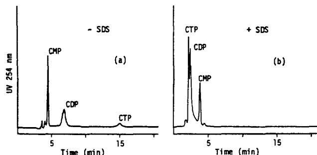
Figure 1. Effect of SDS surfactant on the retention of cytosine nucleotides. Column, 9 \mu m Asahipak GS 320H; mobile phase, (a) 1 mM \text{NaH}_2\text{PO}_4 (pH 3.4), (b) 1 mM SDS (pH 3.4); flow-rate, 2 ml/min; sensitivity, 0.01 a.u.f.s.; temperature, ambient.
