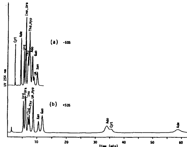
Figure 3. Isocratic elution profiles of a mixture of nucleosides and bases. Mobile phase, (a) aqueous solution (pH 3.4), (b) 1 mM SDS (pH 3.4). Other chromatographic conditions are the same as in Figure 1.
