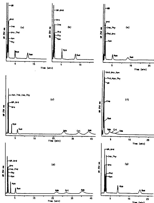
Figure 6. Isocratic elution profiles of a mixture of nucleosides and bases on various silica-based columns. Columns, (a) 5 \mu m PartisSphere C 18 , (b) 5 \mu m PartisSphere C 8 , (c) 5 \mu m Supelcosil LC-CN, (d) 5 \mu m Supelcosil LC-1, (e) 10 \mu m PRP-1, (f) 5 \mu m PartisSphere Silica, (g) 10 \mu m Protesil 300 Octyl. Other chromatographic conditions are the same as in Figure 5.
