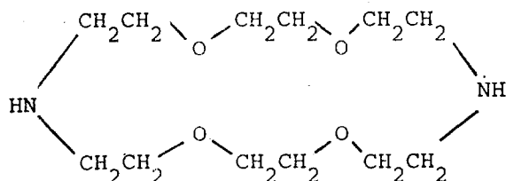
Figure 1. Structure of the Ligand, 1, 7, 10, 16-Tetraoxa-4, 13-Diazacyclooctadecane.
