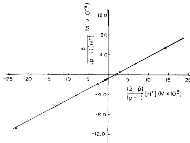
Figure 3. Plot for Titration Data of Ligand according to Eq. 5. \text{L} = 2.500 \times 10^{-3} \text{M} , \text{HCl} = 1.099 \times 10^{-2} \text{M} , I = 0.1 \text{M} \text{N}(\text{CH}_3)_4\text{Cl} at 25^\circ\text{C} .
