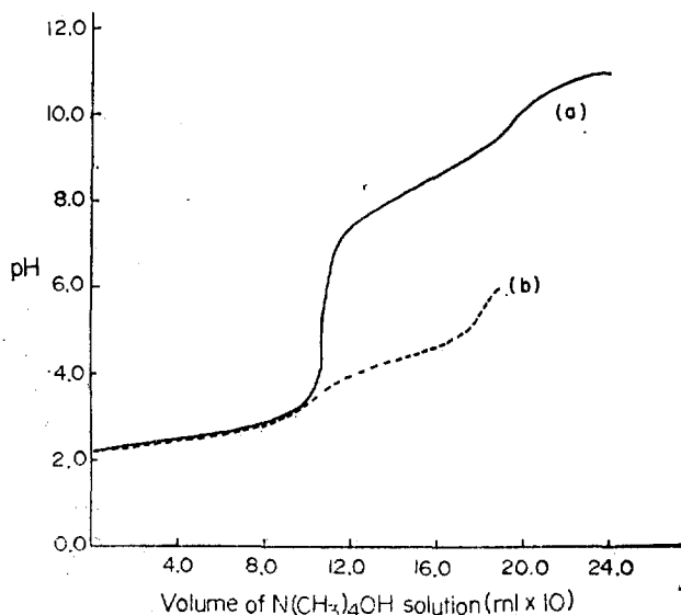
Figure 2. Titration Curves: (a) [\text{L}] = 2.500 \times 10^{-3} \text{M} ; [\text{HCl}] = 1.099 \times 10^{-2} \text{M} ; I = 0.1 \text{M} \text{N}(\text{CH}_3)_4\text{Cl} at 25^\circ\text{C} ; (b) [\text{L}] = n [\text{UO}_2^{2+}] = 2.500 \times 10^{-3} \text{M} ; [\text{HCl}] = 1.099 \times 10^{-2} \text{M} ; I = 0.1 \text{M} \text{N}(\text{CH}_3)_4\text{Cl} at 25^\circ\text{C} . Concentration of \text{N}(\text{CH}_3)_4\text{OH} = 0.1121 \text{M} .
