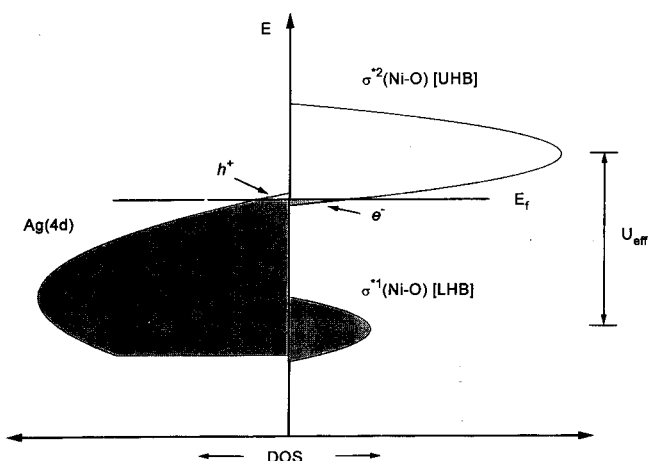
Figure 2. Schematic energy diagram of AgNiO_2 . The antibonding orbital \sigma^*(Ni-O) is separated into two bands, a fulfilled lower Hubbard band (LHB) and an empty upper Hubbard band (UHB) due to the effective intraatomic repulsion energy U_{eff} . The UHB \sigma^{*2}(Ni-O) overlaps with Ag 4d band, generating electrons and holes respectively in each band. 4
