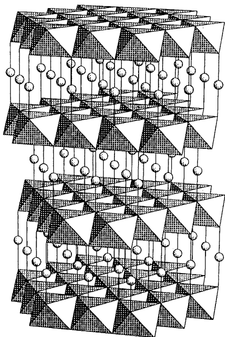
Figure 1. 3R-type delafossite structure of ABO_2 oxides. Balls represent the A^I ions.
