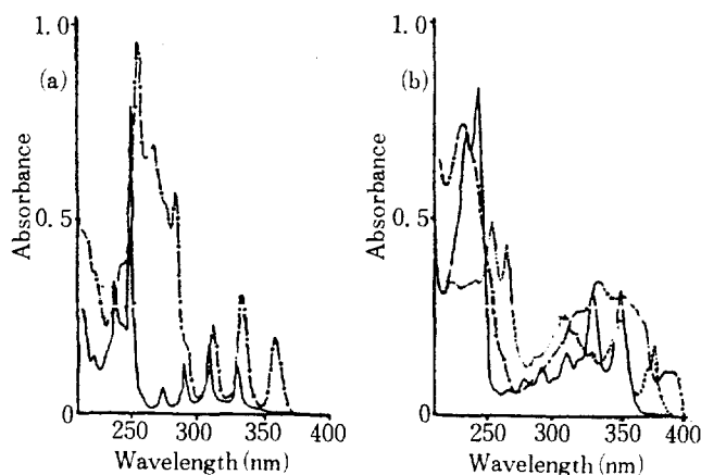
Figure 2. Ultraviolet absorption spectra of 1,6-disubstituted-1,3,5-hexatriynes. (a) \text{Ph}-\equiv\equiv\text{C}-\equiv\text{C}-\text{R} [ \text{R} = \text{Me}(-) , \text{Ph}(- \cdot -) ]. (b) \alpha\text{-Naph}-\equiv\equiv\text{C}-\equiv\text{C}-\text{R} [ \text{R} = \text{Me}(-) , \alpha\text{-Naph}(- - -) , \text{Ph}(\cdot \cdot \cdot) ].
