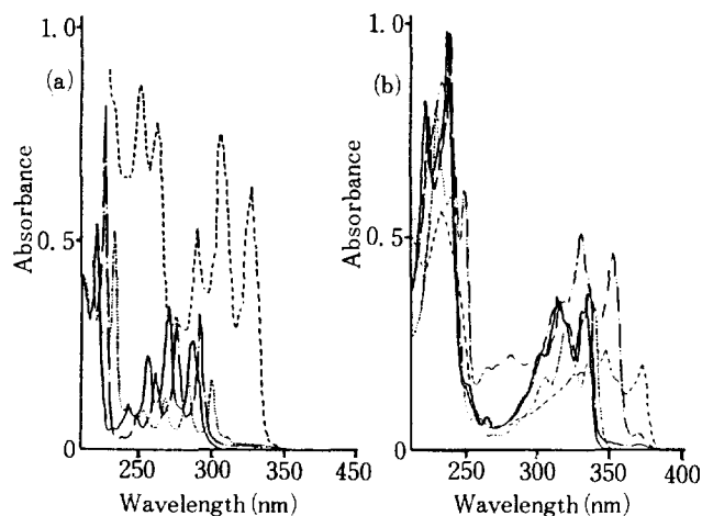
Figure 1. Ultraviolet absorption spectra of 1,4-disubstituted-1,3-butadiynes. (a) \text{Ph}-\equiv\equiv\text{R} [ \text{R} = \text{Me}(-) , \text{t-Bu}(- -) , \text{TMS}(\cdot \cdot \cdot) , \text{Ph}(\text{—}) ]. (b) \alpha\text{-Naph}-\equiv\equiv\text{R} [ \text{R} = \text{Me}(-) , \text{t-Bu}(- -) , \text{TMS}(\cdot \cdot \cdot) , \alpha\text{-Naph}(\text{—}) , \text{Ph}(- \cdot -) ].
