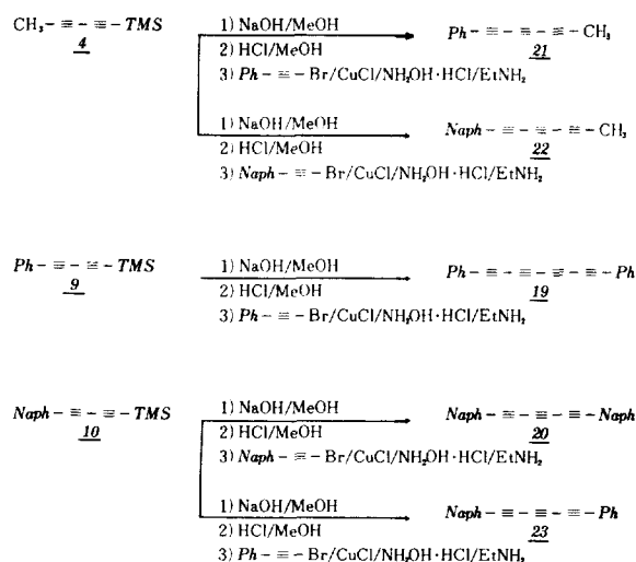
Scheme 2. Synthetic Routes for 1,6-Disubstituted-1,3,5-hexatriynes.
