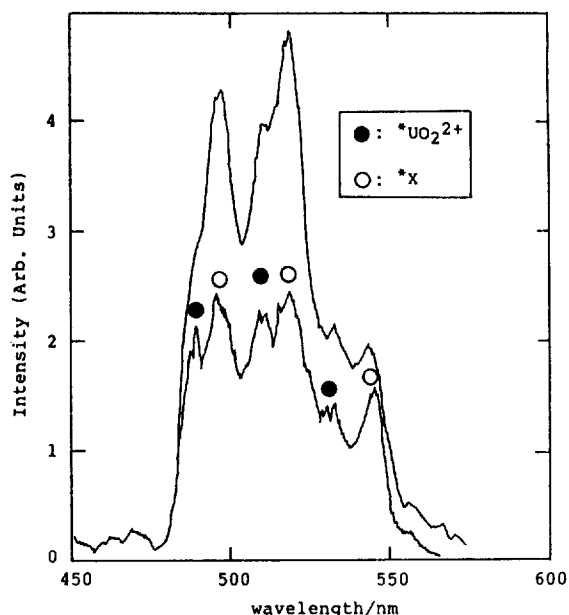
Figure 2. Emission spectra of uranyl ion in aqueous perchlorate solutions at 77 K: [\text{UO}_2^{2+}]_t = 0.01 \text{ M} ; pH = 3.32 and 3.58 (upper) at 25°C.
