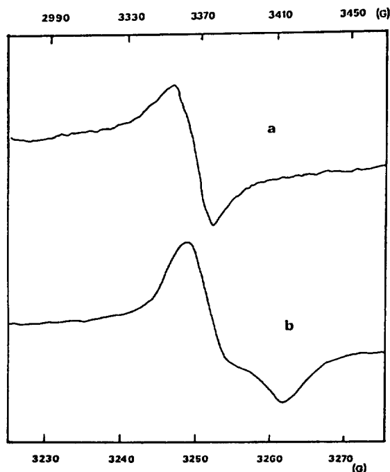
Figure 2. The X-Band EPR spectra of (\text{TTF})_7\text{SbI}_4 at (a) room temperature and (b) 77 K in powder sample.
