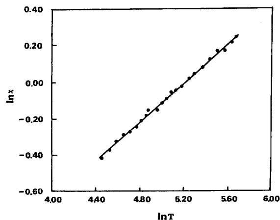
Figure 1. Temperature dependence of magnetic susceptibility for (\text{TTF})_7\text{SbI}_4 .
