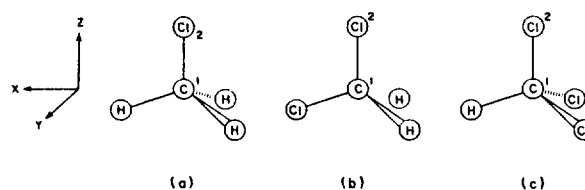
Figure 2. Coordinate systems with the z axes along the respective C-Cl bonds of (a), CH 3 Cl (b), CH 2 Cl 2 and (c), CHCl 3 .
