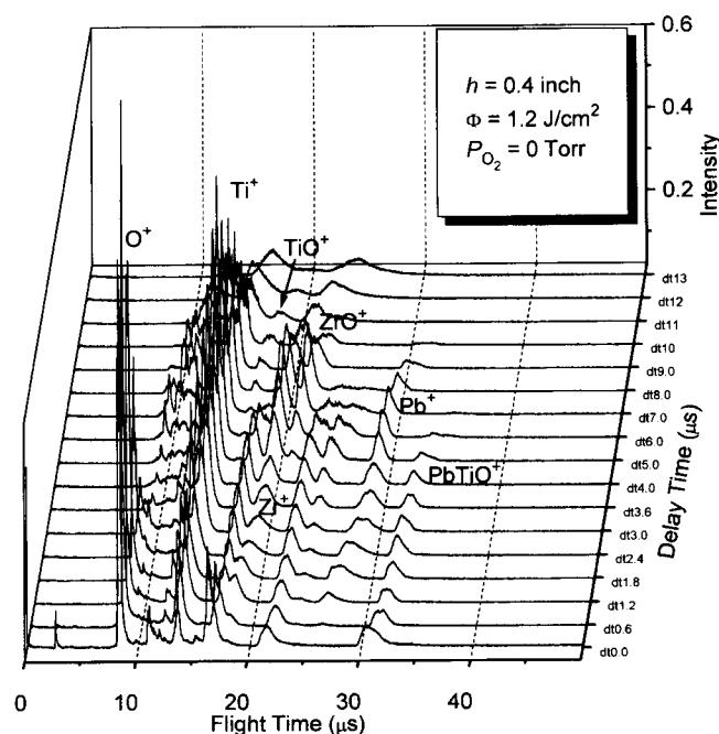
Figure 3. TOF spectra obtained from laser ablation of a PZT target with a laser pulse energy of 1.2 J/cm 2 in high vacuum.
