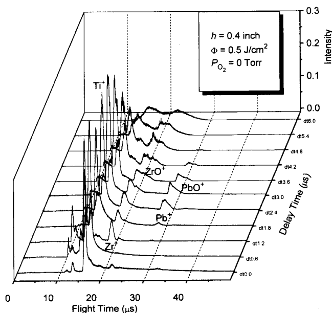
Figure 2. TOF spectra of laser ablated ions from a PZT target in high vacuum as a function of delay time between the laser shot and the extraction pulse: target to extraction zone distance h = 0.4 inch. The ions were ablated by 532 nm with a pulse energy of 0.5 J/cm 2 .
