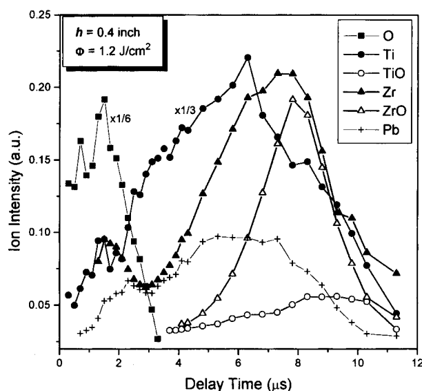
Figure 4. The ion intensities of the ablated species as a function of delay time between the laser irradiation and the extraction pulse at h=0.4 inch following 1.2 \text{ J/cm}^2 laser irradiation of a PZT target. The \text{O}^+ and \text{Ti}^+ ions data was scaled by 1/6 and 1/3, respectively, to facilitate comparison.
