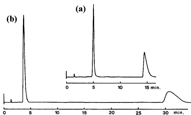
Figure 2. Representative chromatograms for the resolution of N-(3,5-dimethoxybenzoyl) leucine N,N-diethyl amide ( 4h ) on (a) CSP 1 and (b) CSP 2 . See the footnote to Table 1 for the chromatographic conditions.
