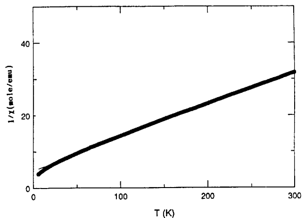
Figure 2. Plot of the inverse susceptibility of \text{Mn}_3(\text{SbTe}_3)_2 as a function of temperature.
