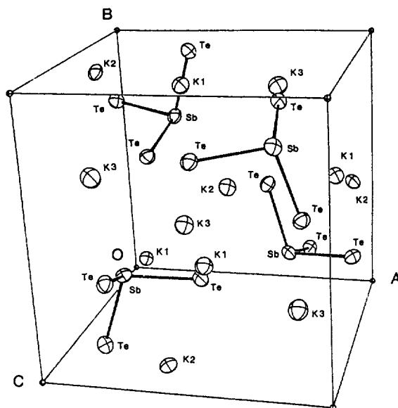
Figure 1. ORTEP diagram of the unit cell of \text{K}_3\text{SbTe}_3 .
