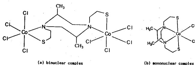
Figure 1. Possible geometry of (a) [\text{Co}_2(\text{medpa})\text{Cl}_8]^{4-} and (b) [\text{Co}(\text{medpa})\text{Cl}_2]^- complexes.
