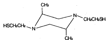
N,N'-bis( \beta -mercaptoethyl)-trans-2,5-dimethylpiperazine (medpa)
