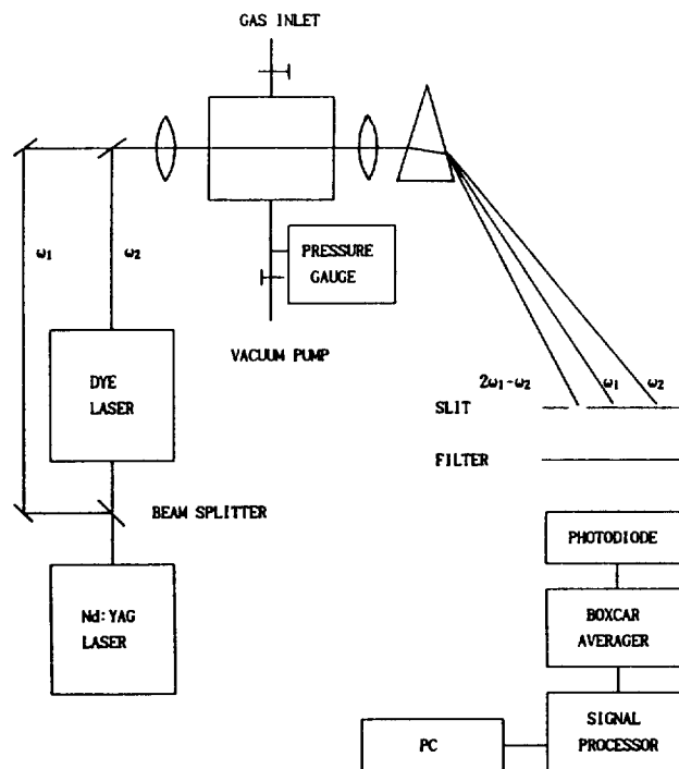
Figure 1. A schematic diagram of the experimental apparatus.
