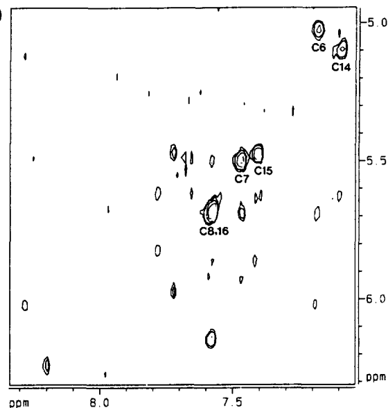
Figure 2. (A) The 500-MHz imino proton spectrum of the psoralen cross-linked DNA in 20 mM phosphate, 200 mM NaCl, \text{H}_2\text{O} , pH 7 at 25^\circ\text{C} ; (B) Expanded region of the NOESY spectrum ( \tau_m = 250 ms) of the psoralen cross-linked DNA in 20 mM phosphate, 200 mM NaCl, \text{D}_2\text{O} , pH 7 at 25^\circ\text{C} , showing the base-sugar \text{H1}' region. The spectrum was acquired with a sweep width of 5050 Hz in both dimensions, 512 t_1 values of 200 scans, and 2 K complex points.
