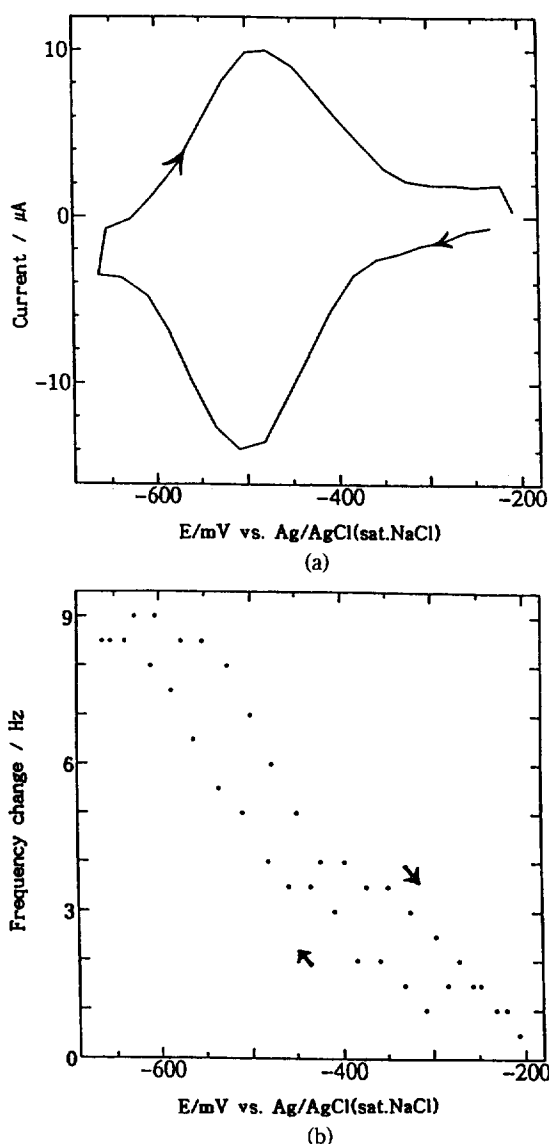
Figure 1. EQCM scan for 10 \mu M C 22 VC 1 in 0.1 M NaTS. (a) Cyclic voltammogram (100 mV/s) and (b) EQCM frequency response for (a).
