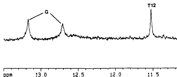
Figure 2. (A) The 500-MHz imino proton spectrum of the psoralen cross-linked DNA in 20 mM phosphate, 200 mM NaCl, \text{H}_2\text{O} , pH 7 at 25^\circ\text{C} ; (B) Expanded region of the NOESY spectrum ( \tau_m = 250 ms) of the psoralen cross-linked DNA in 20 mM phosphate, 200 mM NaCl, \text{D}_2\text{O} , pH 7 at 25^\circ\text{C} , showing the base-sugar \text{H1}' region. The spectrum was acquired with a sweep width of 5050 Hz in both dimensions, 512 t_1 values of 200 scans, and 2 K complex points.
