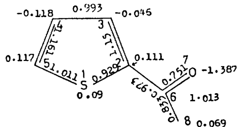
Figure 2. Molecular diagram of 2-Carboxaldehydethiophene.
