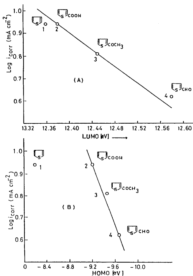
Figure 1. Correlation of LUMO (A) and HOMO (B) energies with \log i_{\text{corr}} . 1) Thiophene; 2) 2-Acetylthiophene; 3) 2-Thiophenecarboxylic acid; 4) 2-Thiophenecarboxaldehyde.
