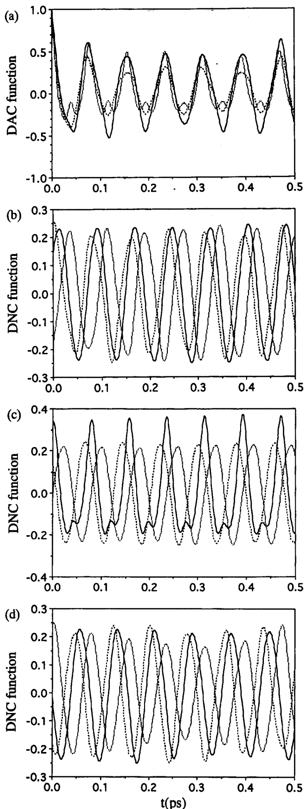
Figure 4. (a) Displacement auto-correlation functions of T (—), O(1) (---), and O(2) (···), and displacement neighbor-correlation functions of (b) T-T (—), T-O(1) (---), and T-O(2) (···), (c) O(1)-T (—), O(1)-O(1) (---), and O(1)-O(2) (···), and (d) O(2)-T (—), O(2)-O(1) (---), and O(2)-O(2) (···) from the center of \alpha -cage at the 8-ring windows in non-rigid zeolite-A framework.
