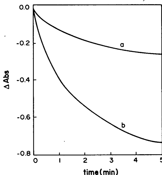
Figure 1. Absorbance ( \Delta\text{Abs} ) changes (at 250 nm) accompanying the reduction of 2 ( 1 \times 10^{-4} \text{ M} ) with \text{NaBH}_4 ( 1 \times 10^{-3} \text{ M} ) in the absence (curve a) and the presence (curve b) of monoclonal antibody JS-I-60 ( 1 \times 10^{-6} \text{ M} ) at pH 8.02 (0.05 M Tris) and 25°C in the presence of 14% (v/v) ethanol.
