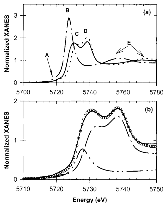
Figure 2. (a) Ce L III -edge XANES spectra for Ce-montmorillonite (—) and reference compounds, Ce(SO 4 ) 2 ·4H 2 O (---) and Ce 2 (SO 4 ) 3 ·8H 2 O (····) (b) Ce L III -edge XANES spectra for Ce-montmorillonite (open circles) and the simulated XANES spectrum (—) based on the weight factor of 0.75 for Ce(SO 4 ) 2 ·4H 2 O (---) and 0.25 for Ce 2 (SO 4 ) 3 ·8H 2 O (····)
