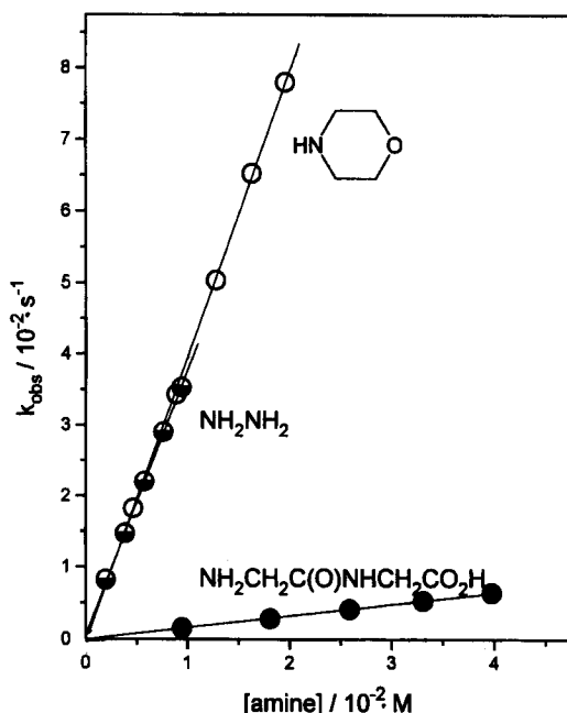
Figure 1. Plots showing dependence of k_{\text{obs}} on amine concentrations for the reaction of 3-butyne-2-one ( 2 ) with glycylglycine (●), hydrazine (○) and morpholine (○) in \text{H}_2\text{O} at 25.0 \pm 0.1 °C.
