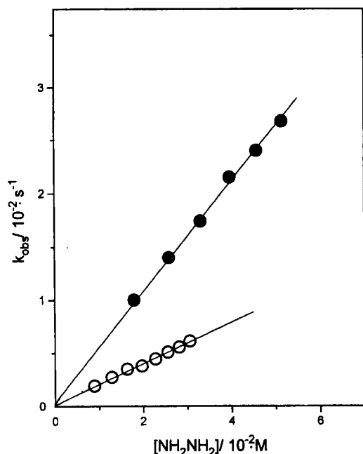
Figure 2. Plots showing kinetic isotope effect for the formation of 3-methylpyrazole (4) from the reaction of 3 with hydrazine in \text{H}_2\text{O} (●) and \text{D}_2\text{O} (○) at 25.0 \pm 0.1^\circ\text{C} .
