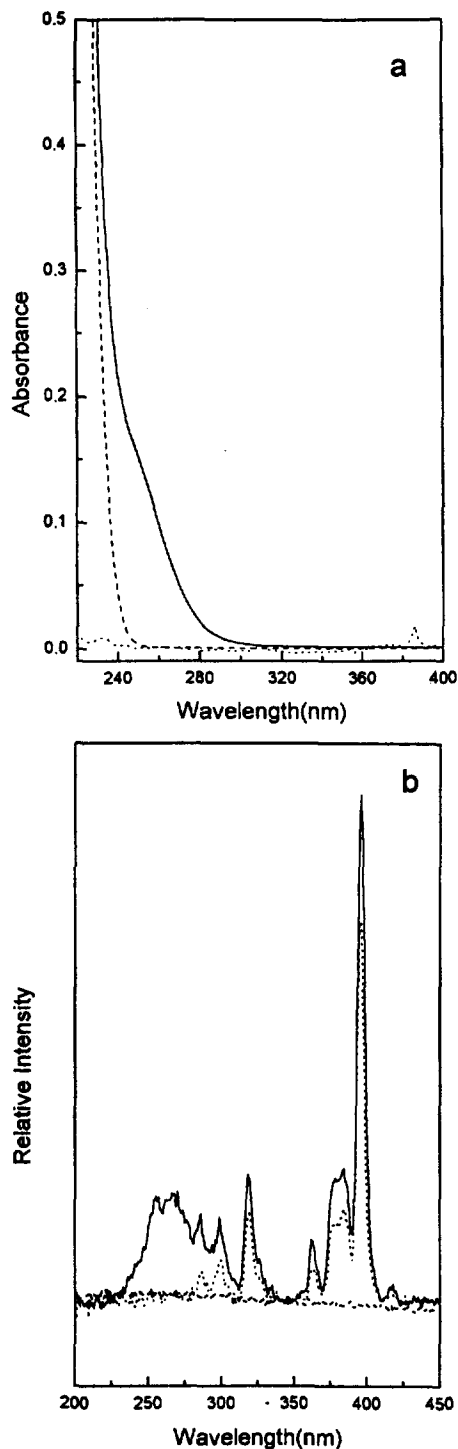
Figure 1. Absorption(a) and excitation(b) spectra of \text{Eu}^{3+} (dotted lines), acetate (dashed lines), and \text{Eu}^{3+} -acetate mixture (solid lines) in aqueous solution. \lambda_{\text{em}} = 595 \text{ nm} . [\text{Eu}^{3+}] = 1.0 \times 10^{-3} \text{ M} , [\text{CH}_3\text{COO}^-] = 0.10 \text{ M} .
