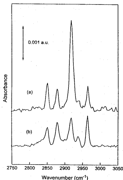
Figure 1. IRA spectra of octadecyl mercaptan monolayers self-assembled, respectively, on (a) gold and (b) silver surfaces.
