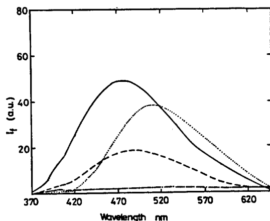
Figure 4. Fluorescence spectra of different species of piroxicam at 298K: (— at H_0 -6.56) cation; (--- at pH 1) neutral; (· · · at pH 7) anion; (- · - · at H_{17.66} ) dianion. \lambda_{ex} = 350 nm.
