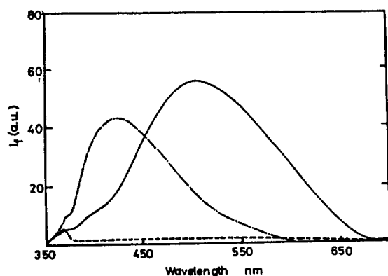
Figure 5. Fluorescence spectra of different species of HMBDC at 298K: (— at H_0 -5.04) cation; (--- at pH 7) neutral; (· · · at H_{17.95} ) anion. \lambda_{ex} = 330 nm.
