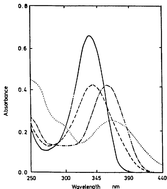
Figure 1. Absorption spectra of different species of piroxicam at 298K: (— at H_0-6.56 ) cation; (--- at pH 2) neutral; (- - - at pH 7) anion; (···· at H_{-17.14} ) dianion.
