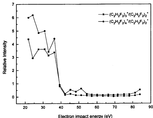
Figure 2. Relative intensity of the (\text{C}_2\text{H}_2\text{F}_2)_n^+ ( n=3, 4 ) to the (\text{C}_2\text{H}_2\text{F}_2)_2^+ depending on the electron impact energy.
