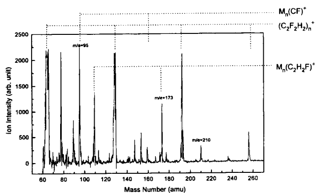
Figure 1. The mass spectrum of 2% 1,1-DFE seeded in 6.5 atm He expansion at 70 eV electron impact energy, \text{M}=\text{C}_2\text{H}_2\text{F}_2 .
