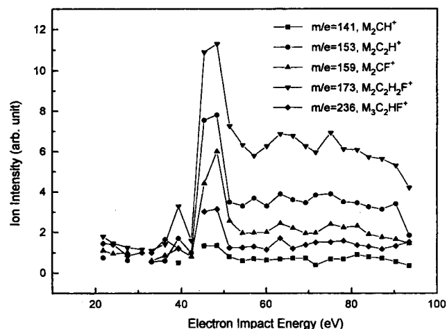
Figure 4. The intensity of the fragment ions as a function of the electron impact energy in the trimer and tetramer, M=\text{C}_2\text{H}_2\text{F}_2 .
