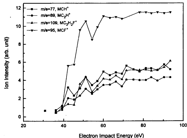
Figure 3. The intensities of the fragment ions as a function of the electron impact energy in the dimer, M=\text{C}_2\text{H}_2\text{F}_2 .
