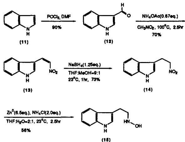
Scheme 4. Synthesis of N-hydroxytryptamine (15).
