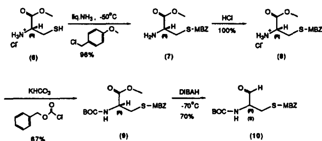
Scheme 3. Synthesis of S-(p-methoxybenzyl)-N-(benzyloxycarbonyl) cysteine aldehyde (10).
