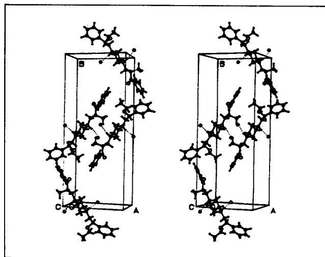
Figure 2. A stereoscopic molecular packing drawing.
