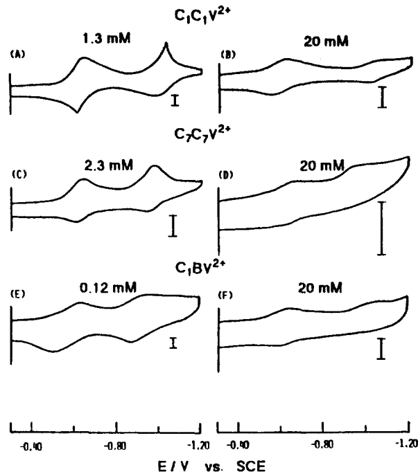
Figure 5. Cyclic voltammograms of 1.0 \times 10^{-3} M C_1C_1V^{2+} (A, B), 1.0 \times 10^{-3} M C_7C_7V^{2+} (C, D) and 0.72 \times 10^{-3} M C_1BV^{2+} (E, F) in the presence of SDS. Scan rates are 130 mV/s. Bars (I) represent 20 \mu A. The concentrations of SDS are shown. (D) was taken at 40^\circ\text{C} and others were at 25^\circ\text{C} .
