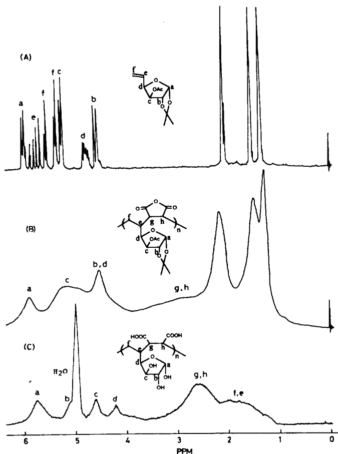
Figure 1. 1 H-NMR spectra: (A) monomer 4 in CDCl 3 , (B) polymer 8 obtained by a bulk polymerization in CDCl 3 , and (C) polymer 11 produced by hydrolysis of polymer 8 in D 2 O and NaOD.
