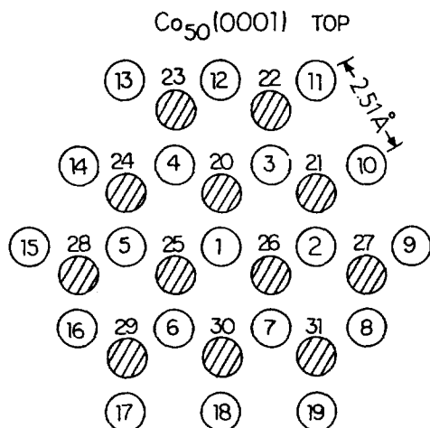
Figure 2. Top view of the Co 50 (0001) cluster with lattices expanded. Empty and shaded circles represent Co atoms of top and middle layer, each. Bottom layer is the repeated top layer 4.0988 Å below (invisible). Layer-layer separations for top-middle and middle-bottom are 2.0494 Å and 2.0494 Å, each.
