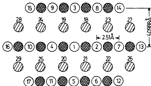
Figure 3. Top view of the Co 43 (10 \bar{1} 0) cluster with lattices expanded. Empty, less-shaded, and more-shaded circles represent Co atoms of top, middle, and bottom layer, each. Layer-layer separations for top-middle and middle-bottom are 0.7246 Å and 1.4491 Å, each.
