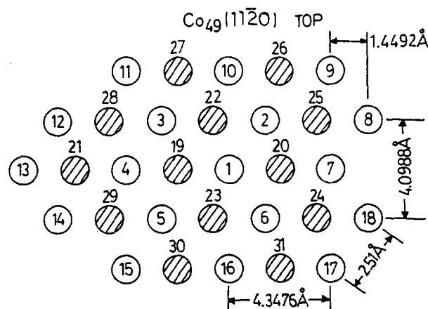
Figure 4. Top view of the Co 49 (11 \bar{2} 0) cluster with lattices expanded. Empty and shaded circles represent Co atoms of top and middle layer, each. Bottom layer is the repeated top layer 2.5100 Å below (invisible). Layer-layer separations for top-middle and middle-bottom are 1.255 Å and 1.255 Å, each.
