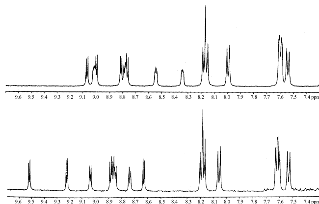
Figure 1. Partial 400 MHz proton NMR spectra of corrole ( 9 ) (bottom) and ( 11 ) (top) in CDCl 3 . The meso -tolyl groups have almost identical chemical shifts while the \beta -pyrrolic and \beta -furyl signals show large differences.
